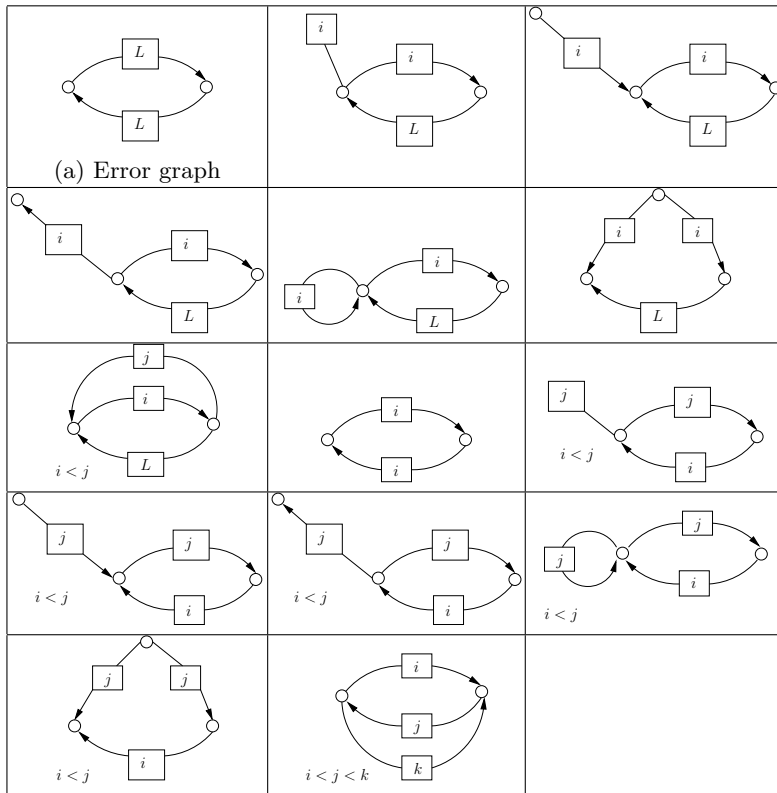
Fig. 4: Leader election (forbidden minors).
